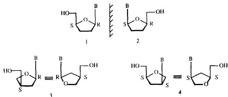
Figure 1. General structure representations of dideoxynucleosides, 1 and 2 , dideoxyanionucleosides, 3 , and isodideoxynucleosides, 4 .
