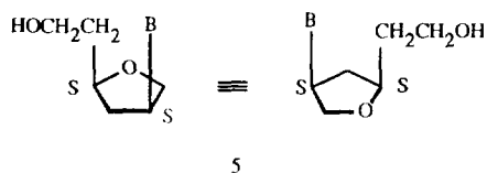
Figure 2. Structural Representations of Homologous Isodideoxynucleosides
